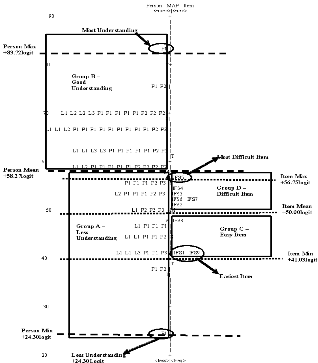
Figure 2: Wright Map
